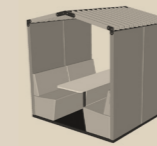
Six Person Pitched Roof H2135 x W2000 x D1800 x SH440mm Table Height: 715mm
